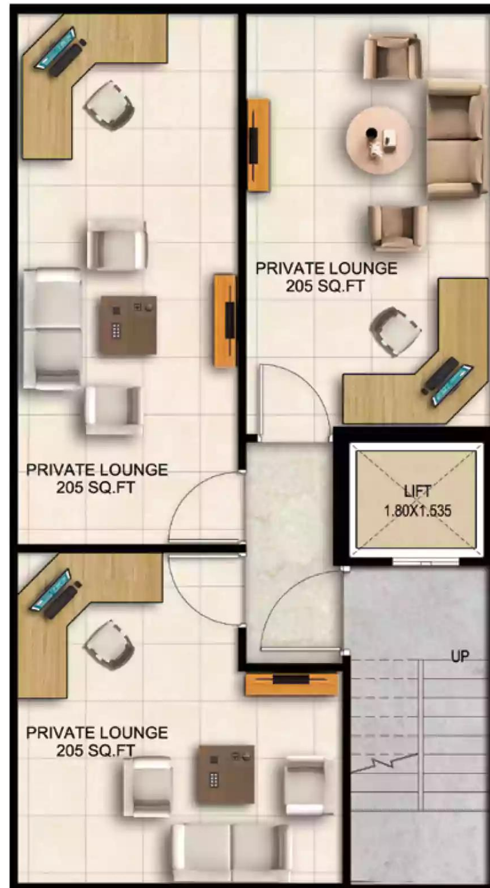
Basement Plan
